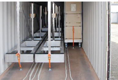
In this 40 feet container are wing parts for the Airbus transports
